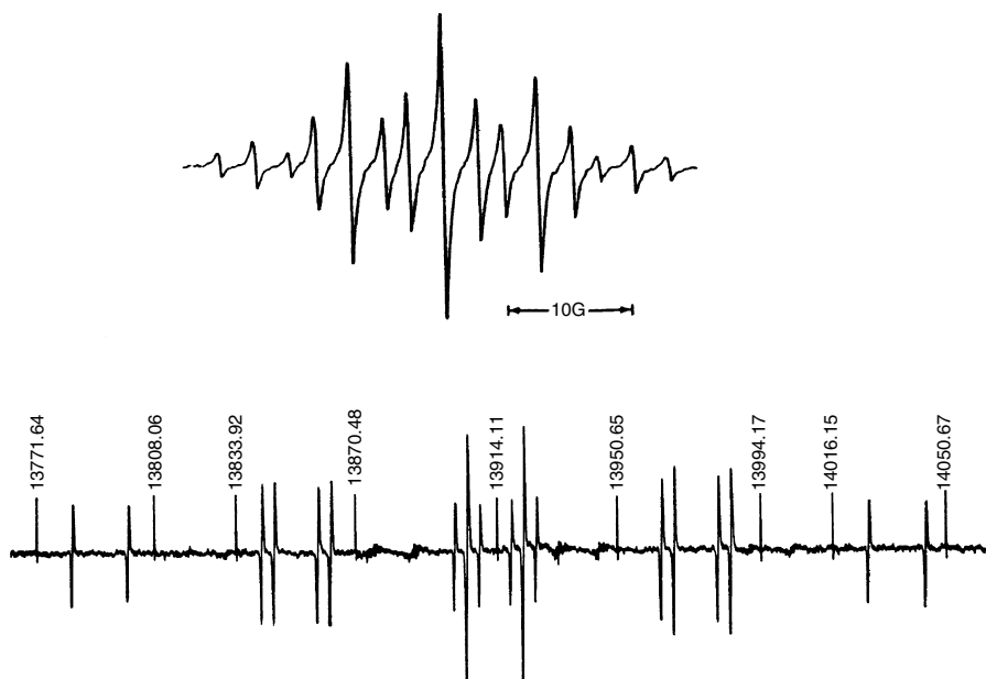
Fig. 11.P11. (a) ESR spectrum of butadiene radical anion from J. Chem. Phys. 41 , 1062 (1964); (b) ESR spectrum of allyl radical from J. Am. Chem. Soc. , 90 , 7157 (1968).
