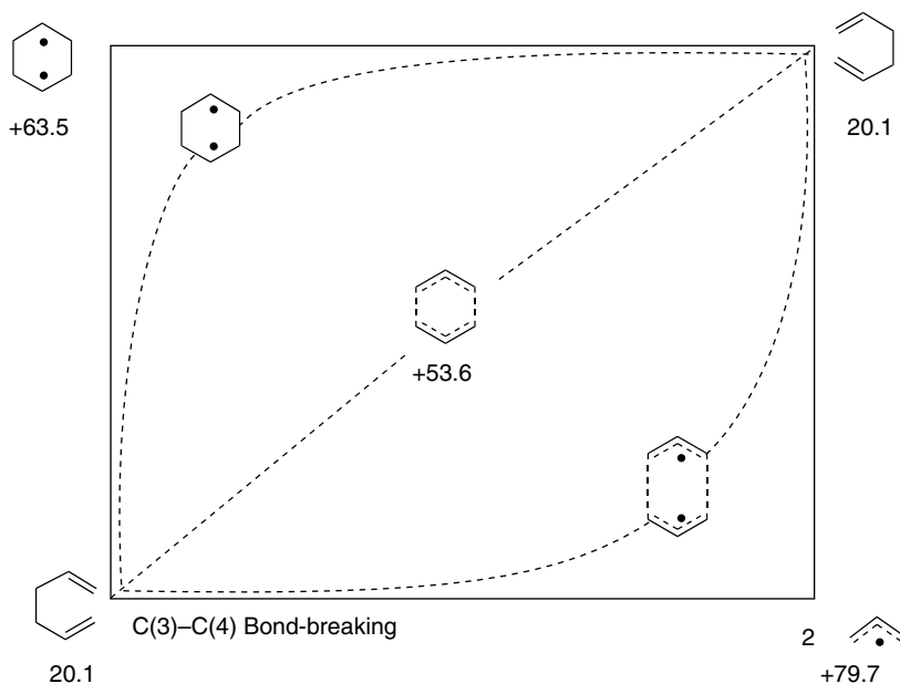
Fig. 10.38. More-O'Ferrall-Jencks diagram representing the variable transition structure for the Cope rearrangement. Energies (in kcal/mol) are from thermodynamic data, as quoted by D. A. Hrovat, J. Chen, K. N. Houk, and W. T. Borden, J. Am. Chem. Soc. , 122 , 7456 (2000).
