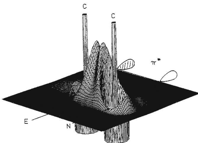
Fig. 1.40. Perspective of Laplacian -\nabla^2\rho_e(r) of ethene in a plane perpendicular to the molecular plane. From E. Kraka and D. Cremer in The Concept of the Chemical Bond , Z. B. Maksic, ed., Springer-Verlag 1990, p. 533.
