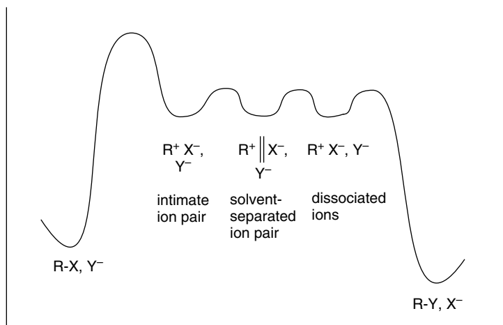
Fig. 4.4. Schematic relationship between reactants, ion pairs, and products in substitution proceeding through ion pairs.
