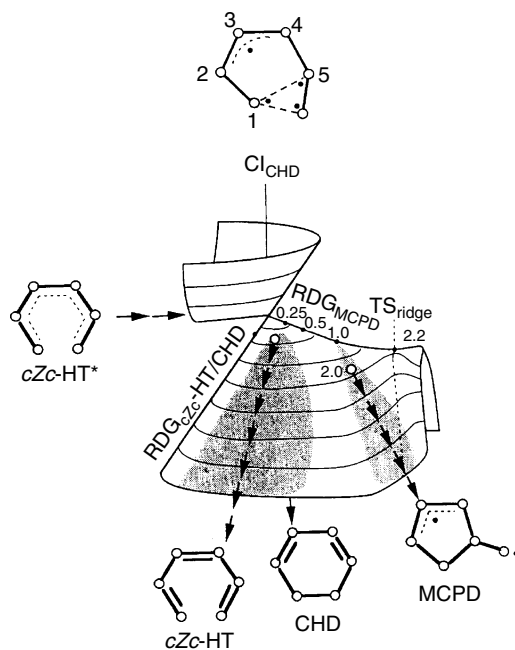
Fig. 12.31. Schematic representation of conical intersection showing partitioning between 1,3-hexatriene, 1,3-cyclohexadiene, and bicyclo[3.1.0]hex-2-ene products. Reproduced from J. Phys. Chem. A , 101 , 2023 (1997), by permission of the American Chemical Society.
