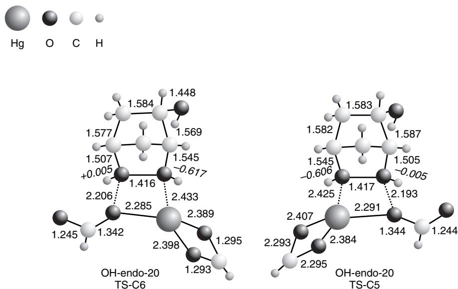
Fig. 5.5. Transition structures for C(6) and C(5) mercuriation of the endo hydroxy derivative of norbornene. Italic numbers give the NPA charges at the reacting carbons. Reproduced from J. Org. Chem. , 66 , 5182 (2001), by permission of the American Chemical Society.
