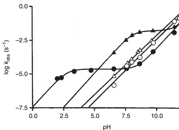
Fig. 7.P28. pH-Rate plots for thioesters 28-A (○), 28-B (●), 28-C (▲) and 28-D (△). Reproduced from J. Org. Chem. , 62 , 4816 (1997), by permission of the American Chemical Society.
