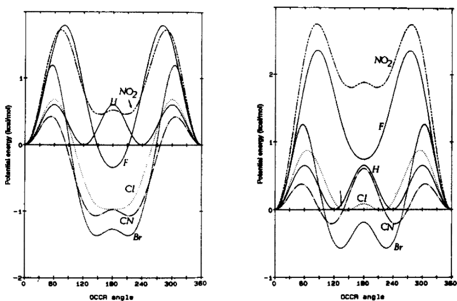
Fig. 2.22P. (a) Rotational profile of the isolated molecules. (b) Rotational profile in solvent cavity with dielectric constant 4.7. Reproduced by permission of Elsevier.
