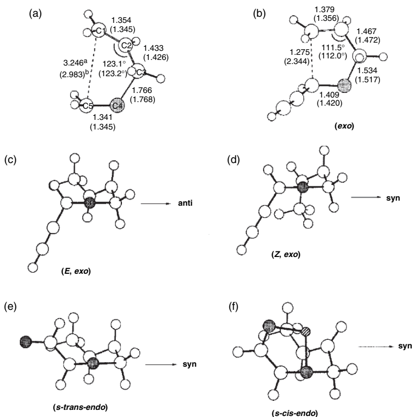
Fig. 10.40. Relationship between TS structure and stereoselectivity in [2,3]-sigmatropic rearrangement of allyloxycarbanions: (a) early TS for unsubstituted allyloxymethyl anion; (b) tighter cyclic TS for stabilized allyloxypropargyl anion; (c,d) preferred conformation of E - and Z -crotyloxypropargyl anions leading to the E → anti and Z → syn stereoselectivity; (e,f) unchelated and chelated TSs for \alpha -crotyloxy ethanal enolate leading to the E → syn stereoselectivity. Reproduced from Tetrahedron , 50 , 5917 (1994), by permission of Elsevier.
