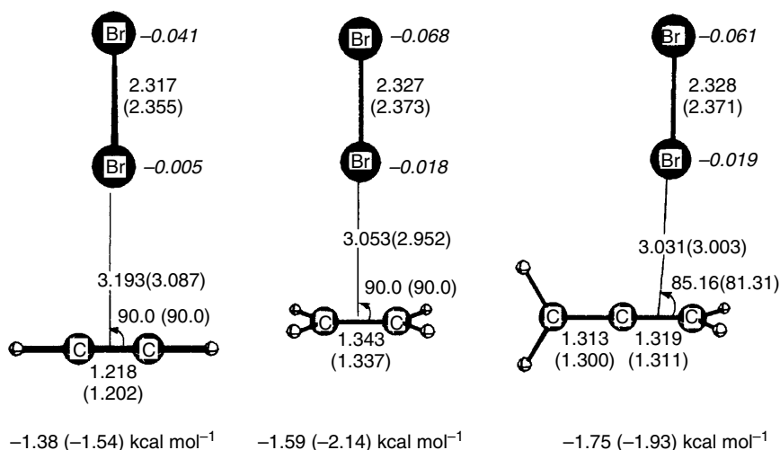
Fig. 5.10. Optimized structures and \Delta E for formation of (a) ethyne-Br 2 , (b) ethene-Br 2 , and (c) allene-Br 2 complexes. Values of \Delta E from MP2/6-311+G** and B3LYP/6-311G** (the latter in parentheses). Reproduced from Chem. Eur. J. , 967 (2002), by permission of Wiley-VCH.
