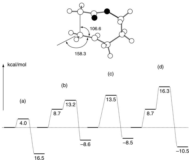
Fig. 11.10. Comparison of energies of (a) 8- endo-s-cis , (b) 8- endo-s-trans , (c) 7- exo-s-cis , and (d) 7- exo-s-trans transition structures. Reproduced from J. Am. Chem. Soc. , 120 , 7469 (1998), by permission of the American Chemical Society.
