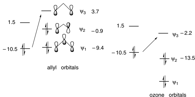
Fig. 1.23. Comparison of FMO interactions of ethene with an allyl anion and ozone.
