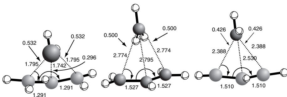
Fig. 10.34. Transition structures for suprafacial 1,3-migrations of BH 2 (left), CH 3 (center), and NH 2 (right) at the QCISD/6-311+G** level. Bond distances and NPA bond orders are shown. Adapter from J. Phys. Chem. A , 106 , 5709 (2002), by permission of the American Chemical Society.
