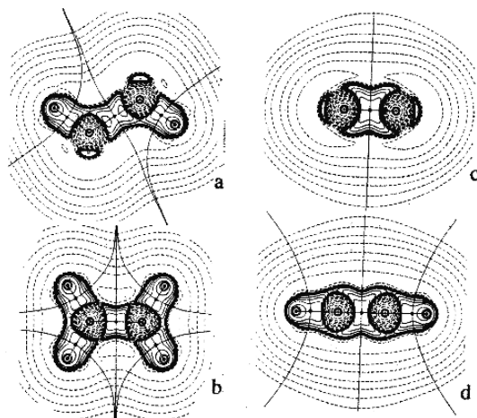
Fig. 1.39. Contour maps of L(r) for: (a) ethane in a plane bisecting anti -hydrogens; (b) ethene in the molecular plane; (c) ethene perpendicular to the molecular plane, and (d) ethyne. The solid lines depict the zero-flux surfaces of the C and H atoms. From J. Phys. Chem. 100 , 15398 (1996).
