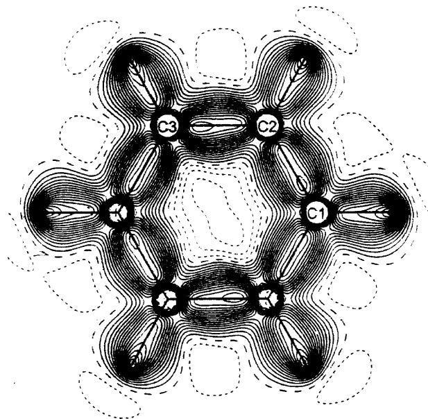
Fig. 1.24. Deformation electron density in the molecular plane of benzene. Contours at 0.05e\text{\AA}^{-3} intervals. Positive contours are solid; negative contours are dashed. From Chem. Eur. J. , 8 , 3512 (2002).
