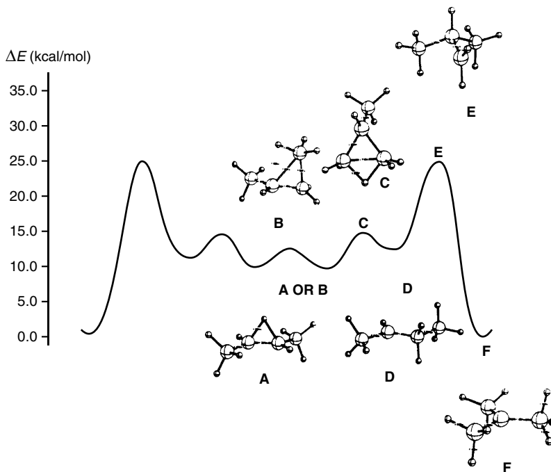
Fig. 4.11. Energy profile for the scrambling and rearrangement of C_4H_9^+ cation. (A) H-bridged; (B) methyl-bridged; (C) edge protonated methylcyclopropane; (D) classical secondary; (E) classical primary; (F) tertiary. Adapted from J. Am. Chem. Soc. , 112 , 4064 (1990); J. Am. Chem. Soc. , 115 , 259 (1993) and J. Phys. Chem. , 100 , 633 (1996), by permission of the American Chemical Society.
