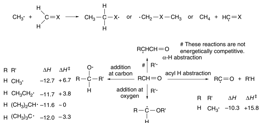
Fig. 11.8. G3(MP2) computational \Delta H and \Delta H^\ddagger in kcal/mol for reactions of alkyl radicals with aldehydes.
