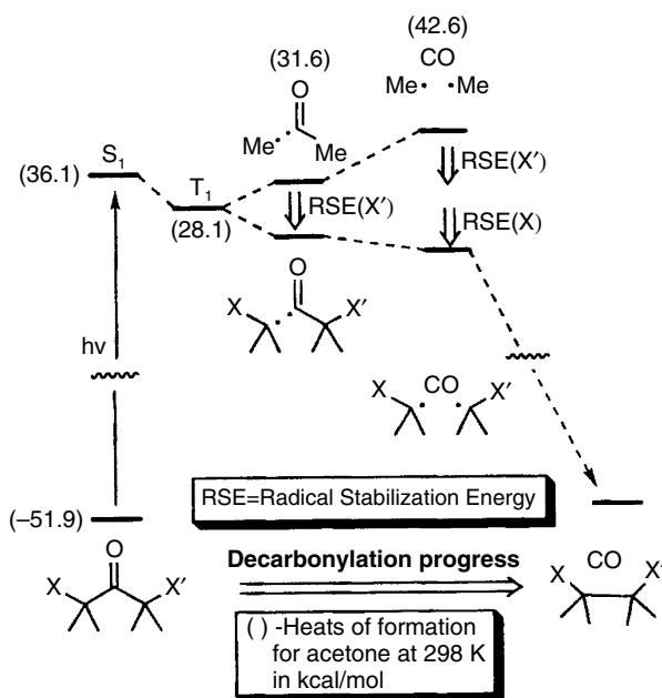
Fig. 12.23. Energetics for \alpha -cleavage and decarbonylation of acetone showing the effect of radical stabilization. Reproduced from J. Org. Chem. , 67 , 3749 (2002), by permission of the American Chemical Society.
