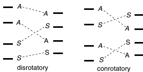
Fig. 10.24. Correlation diagrams for interconversion of cyclobutene and 1,3-butadiene: (left) symmetry forbidden disrotatory reaction; (right) symmetry allowed conrotatory reaction.
