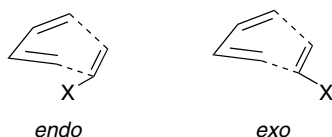
Fig. 10.3. Exo and endo transition structures for the Diels-Alder reaction.
