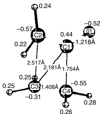
Fig. 10.20. Bond distances and NPA charges for the DFT (BP86/III) transition structure for addition between ketene and ethene. Reproduced from J. Phys. Chem. A , 106 , 431 (2002), by permission of the American Chemical Society.
