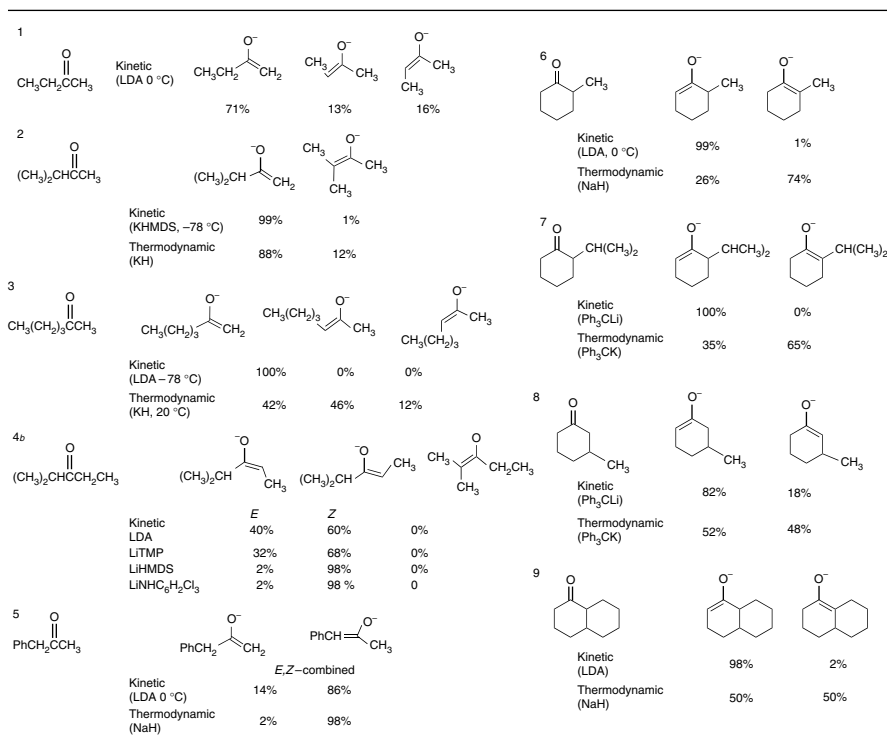
Scheme 6.1. Composition of Enolate Mixtures Formed under Kinetic and Thermodynamic Control a
