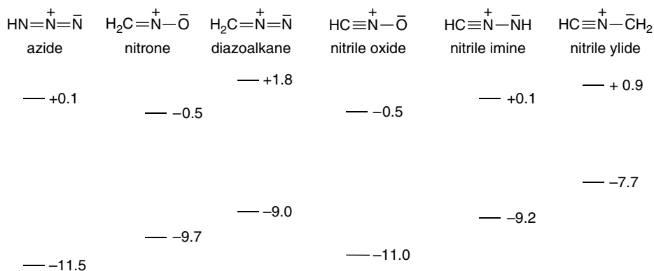
Fig. 10.14. Estimated energies (eV) of frontier \pi MOs for some 1,3-dipoles. Data from J. Am. Chem. Soc. , 95 , 7287 (1973).
