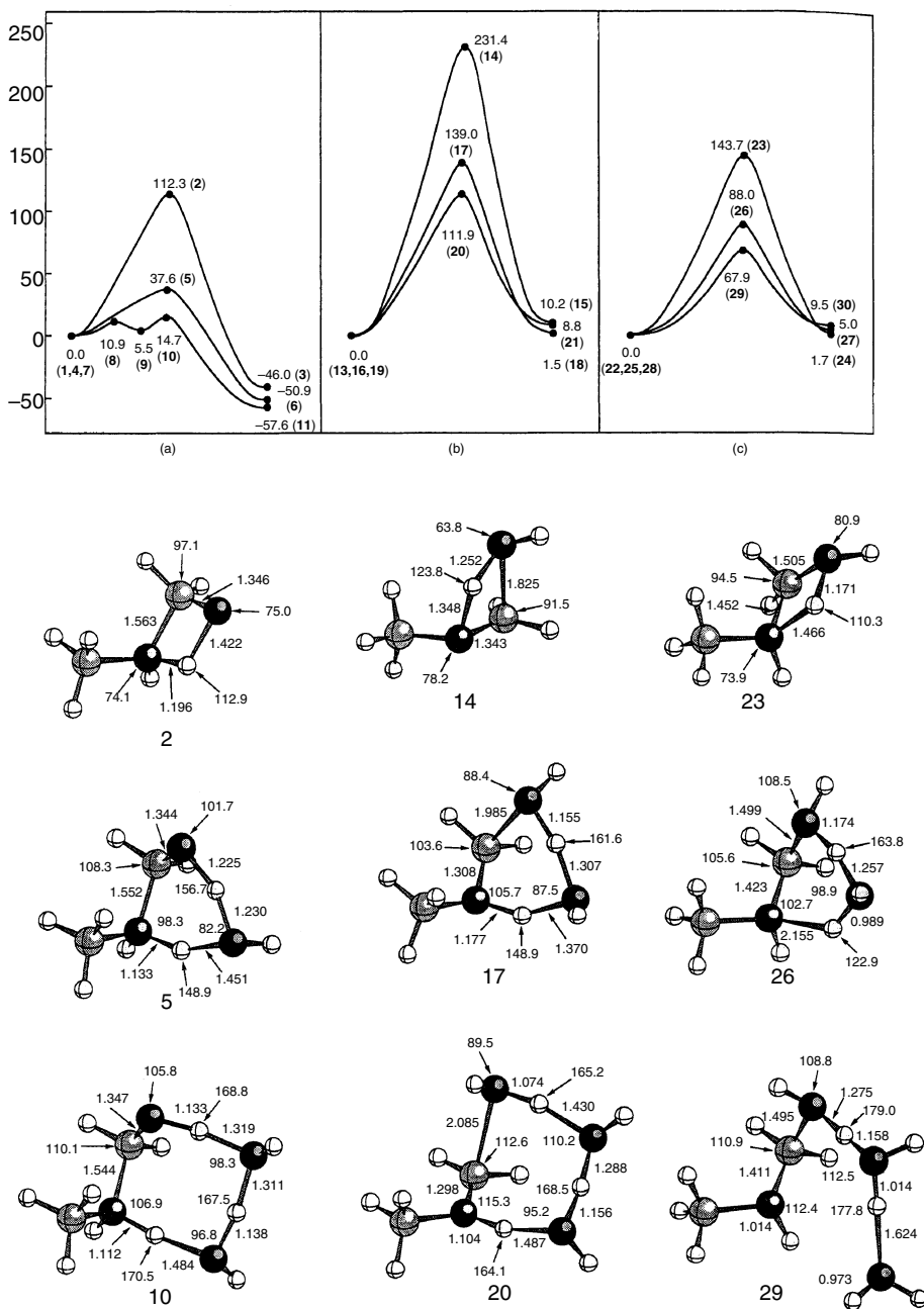
Fig. 7.7. Upper panel: Energy profiles from G2 computations for: (a) carbinolamine formation, (b) imine formation, and (c) iminium ion formation with zero, one, and two water molecules. Lower panel: Transition structures for carbinolamine, imine, and iminium ion formation with zero, one, and two water molecules and showing selected bond lengths and angles. Reproduced from J. Phys. Chem. A , 102 , 4930 (1998), by permission of the American Chemical Society.
