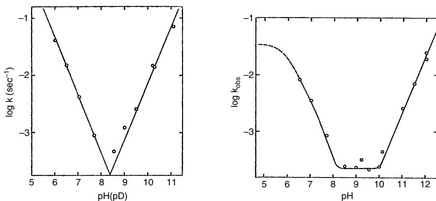
Fig. 7.8. pH-Rate profiles for formation of oximes of benzaldehyde (left) and acetone (right). The solid lines are the theoretical lines of slope -1 , 0 , and +1 . Reproduced from J. Am. Chem. Soc. , 88 , 2508 (1966), by permission of the American Chemical Society.
