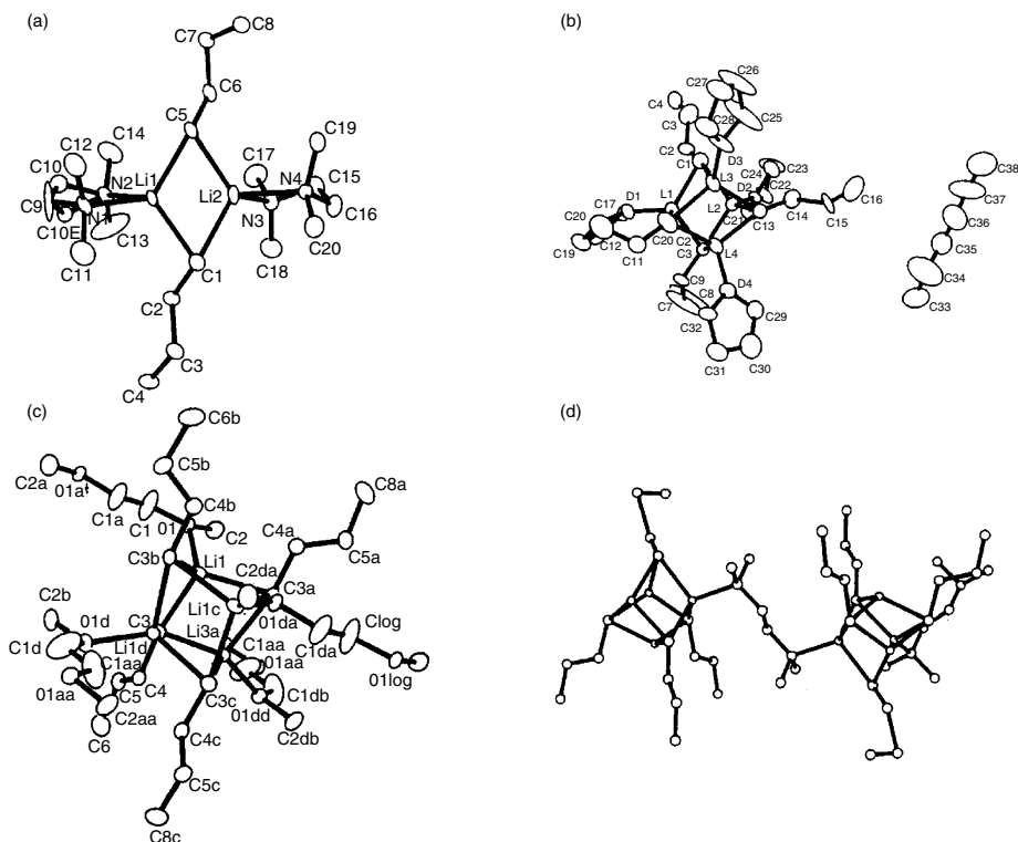
Fig. 6.2. Crystal structures of n -butyllithium: (a) [(n\text{-BuLi-TMEDA})_2]_2 ; (b) [(n\text{-BuLi-THF})_4]\text{hexane} ; (c) [(n\text{-BuLi-DME})_4] ; (d) [(n\text{-BuLi})_4\text{.TMEDA}] . Reproduced from J. Am. Chem. Soc. , 115 , 1568, 1573 (1993), by permission of the American Chemical Society.
