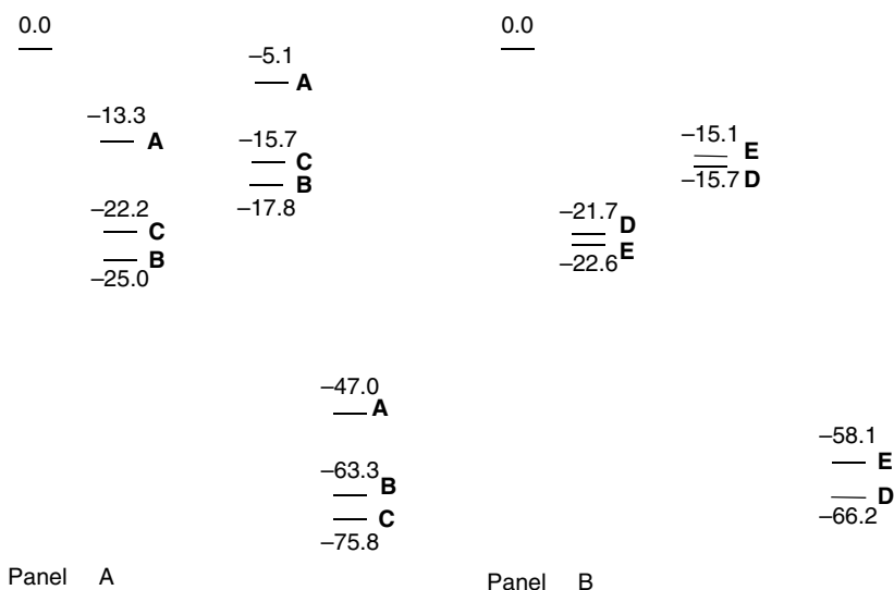
Fig. 7.14. Panel A: Relative \Delta H of reactant complex, transition structure, and products at 0°C (including ZPE correction) for acetone ( A ), methoxyacetone ( B ), and methoxyacetaldehyde ( C ). Panel B: Relative \Delta H at 0°C (including ZPE correction) for 3-methoxypropanal ( D ) and 4-methoxy-2-butanone ( E ). Data from J. Am. Chem. Soc. , 117 , 5055 (1995).
