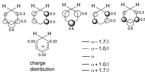
Fig. 9.2. \pi Molecular orbitals and energy levels for the cyclohexadienylum ion.
