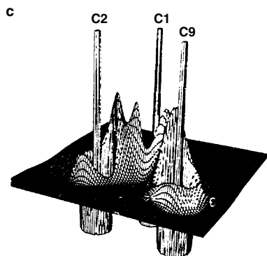
Fig. 8.P14. (a) Bond lengths and (b) inter-ring angles for minimum-energy cation; (c) -\nabla^2\rho(\mathbf{r}) in the \text{C}(1)\text{--C}(2)\text{--C}(9) plane. Reproduced by permission of the American Chemical Society Bond Orders: 1,2: 1.04; 2,3: 1.59; 3,4: 1.57; 1,6: 0.94; 1,9: 1.04; 8,9: 1.56; 2,9: 0.34.
