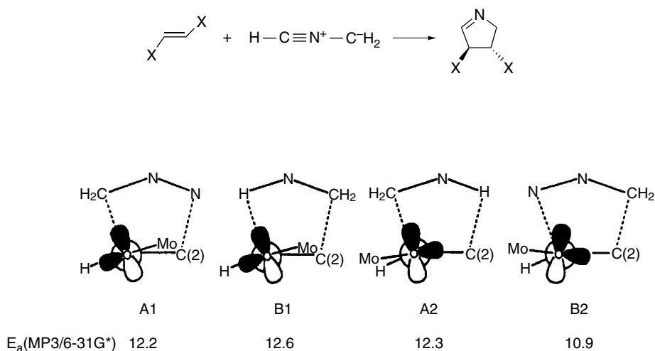
Fig. 10.17. Transition structures for 1,3-dipolar addition of methoxyethene and diazomethane. Structures A1 and B1 correspond to the syn conformation of methoxyethene, whereas A2 and B2 correspond to the anti conformation. The TS with the lowest energy corresponds to the observed product. From J. Chem. Soc., Faraday Trans. , 90 , 1077 (1994).
