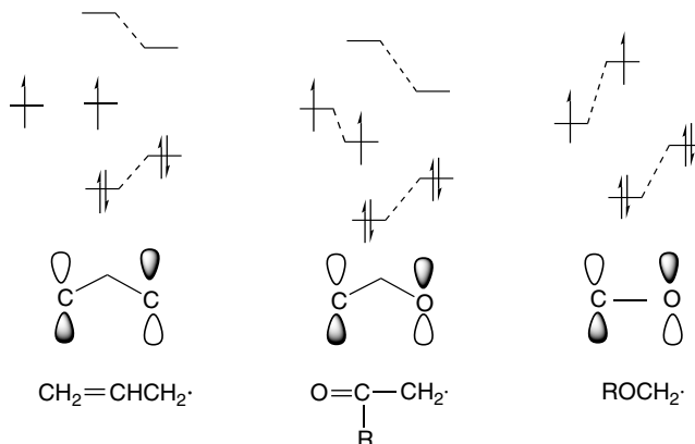
Fig. 3.19. PMO representation of p -orbital interactions with (a) C=C , (b) C=O , and (c) OR substituents. The form of the resulting SOMO is shown at the bottom.
