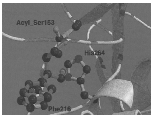
Fig. 2.30. Active site model of PPL showing the binding of 2-phenylpentane-1,4-diol in an active site. Note the \pi - \pi stacking with Phe-216 and placement of the C(4) hydroxyl near the acyl serine-153 residue. Reproduced from Tetrahedron , 55 , 14961 (1999), by permission of Elsevier. (See also color insert.)
