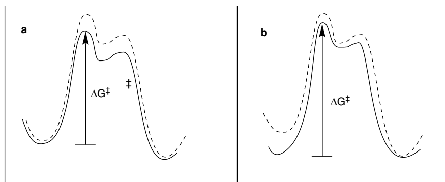
Fig. 4.2. Solid line: polar solvent; dashed line: nonpolar solvent. (a) Solvent effects on R-X \rightarrow R^+ + X^- . Polar solvents increase the rate by stabilization of the R^{\delta+}\cdots X^{\delta-} transition state. (b) Solvent effect on R-X^+ \rightarrow R^+ + X . Polar solvents decrease the rate because stabilization of R^{\delta+}\cdots X^{\delta-} transition state is less than for the more polar reactant.
