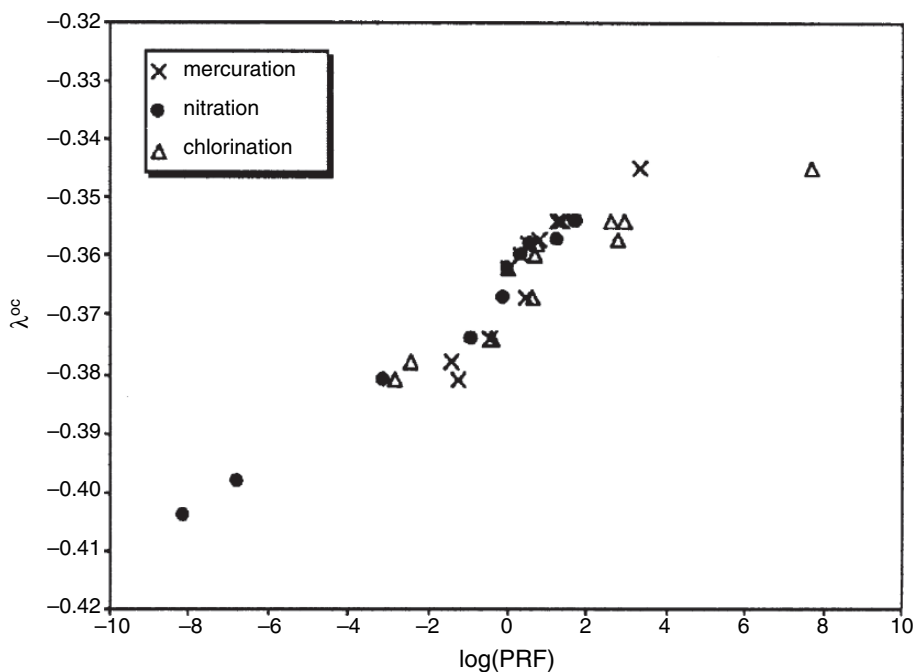
Fig. 9.6. Correlation between the interaction energy \lambda^{oc} and the log of partial rate factors for mercuration, nitration, and chlorination. Reproduced from J. Phys. Chem. A , 107 , 2875 (2003), by permission of the American Chemical Society.
