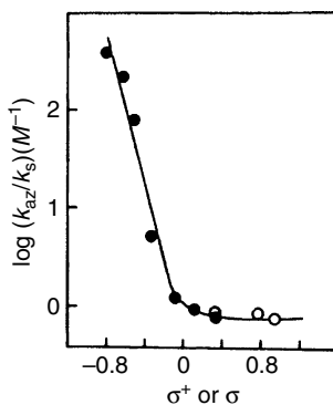
Fig. 4.P20. Log of product selectivity (k_{\text{az}}/k_{\text{s}})\text{M}^{-1} versus \sigma^+ . Solid circles are substituted benzoate leaving groups and open circles are chloride. Reproduced from J. Am. Chem. Soc. , 113 , 5 871 (1991), by permission of the American Chemical Society.
