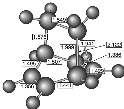
Fig. 12.24. Structure of conical intersection for benzene + ethene addition from J. Am. Chem. Soc. , 118 , 7353 (1996), by permission of the American Chemical Society.
