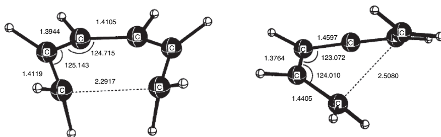
Fig. 10.26. Disrotatory (left) and conrotatory (right) transition structures for 1,3,5-hexatriene electrocycyclization from MP2/CAS/6-311+G( d,p ) calculations. Reproduced from J. Phys. Chem. A , 103 , 2878 (1999), by permission of the American Chemical Society.
