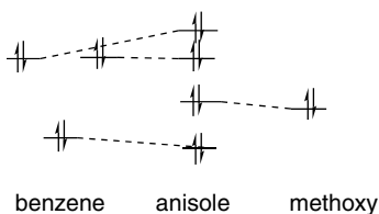
Fig. 9.3. MO diagram for anisole (methoxybenzene) showing effects of methoxy substituent.
