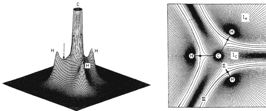
Fig. 1.28. (a) Electron density of the methyl cation in the plane of the atoms (truncated at C); (b) gradient vector field \nabla\rho(\mathbf{r}) of the electron density distribution terminating at H ( I_H ), C ( I_C ); the bond path and critical point (II); and the zero flux surfaces (III) partitioning the ion into C and H atoms. From E. Kraka and D. Cremer, in Theoretical Models of Chemical Bonding , Part 2, Z. B. Maksic, ed., Springer Verlag, Berlin, 1990, pp. 459, 461.
