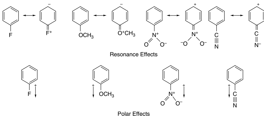
Fig. 3.26. Resonance and polar effects of representative substituents.
