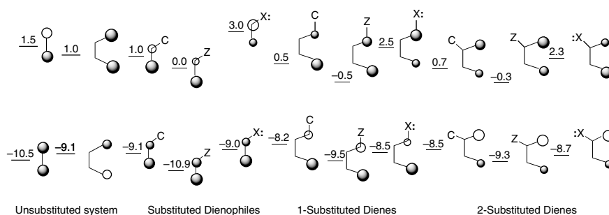
Fig. 10.5. Coefficients and relative energies of dienophile and diene frontier MOs. Orbital energies are given in eV. The sizes of the circles give a relative indication of the orbital coefficient. Z stands for a conjugated EWG, e.g., C=O, C≡N, NO 2 ; C is a conjugated substituent without strong electronic effect, e.g., phenyl, vinyl; X is a conjugated ERG, e.g., OCH 3 , NH 2 . From J. Am. Chem. Soc. , 95 , 4092 (1973).
