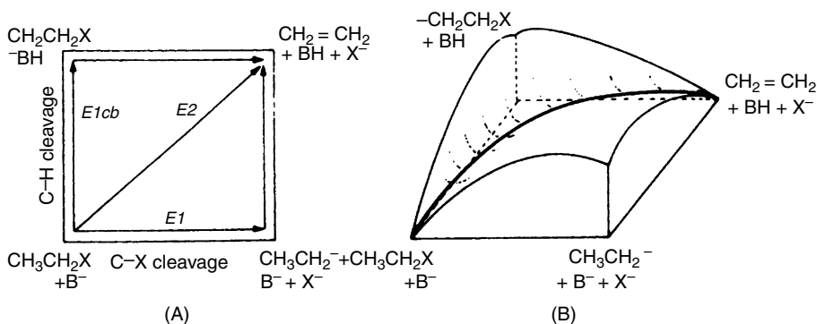
Fig. 5.12. Two-dimensional potential energy diagrams depicting E1, E2, and E1cb mechanisms.
