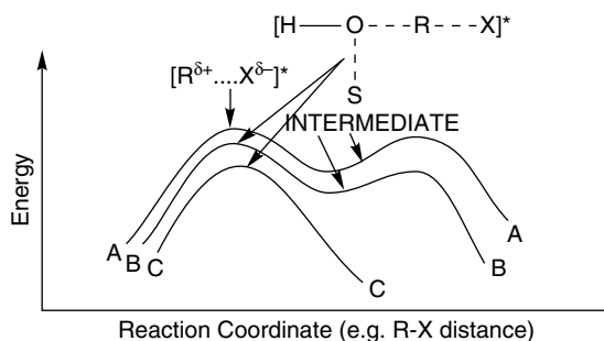
Fig. 4.5. Reaction energy profiles for substitution mechanisms. A is the S_N1 mechanism. B is the S_N2 mechanism with an intermediate ion pair or pentacoordinate species. C is the classical S_N2 mechanism. Reproduced from T. W. Bentley and P. v. R. Schleyer, Adv. Phys. Org. Chem. , 14 , 1 (1977), by permission of Academic Press.
