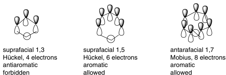
Fig. 10.31. Classification of sigmatropic hydrogen shifts with respect to basis set orbitals.
