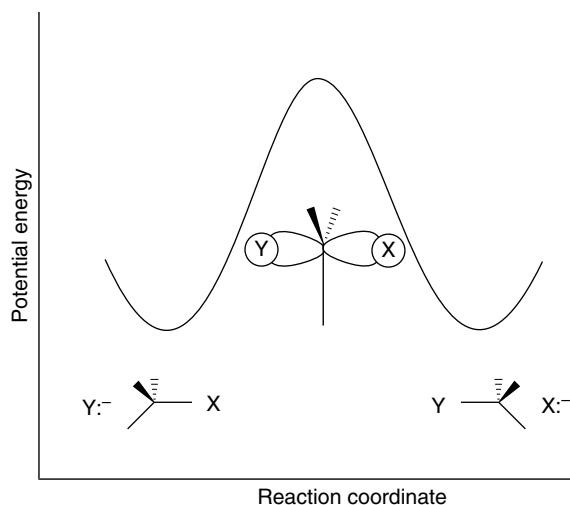
Fig. 4.3. Reaction energy profile for nucleophilic substitution by the direct displacement ( S_N2 ) mechanism.
