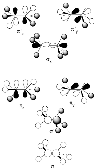
Fig. 1.34. Molecular orbitals of ethane revealing \pi character of \pi_z , \pi_y , \pi'_z , and \pi'_y orbitals. Only filled orbitals are shown.
