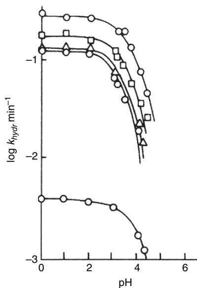
Fig. 7.P25. pH-Rate profile for the hydrolysis of alkyl N -methylmaleamic acids at 39°C. The order of increasing reactivity is R^1 = H < Me < Et < i\text{-Pr} \ll t\text{-Bu} . Reproduced from J. Chem. Soc., Perkin Trans. 2 , 1206 (1972), by permission of the Royal Society of Chemistry.
