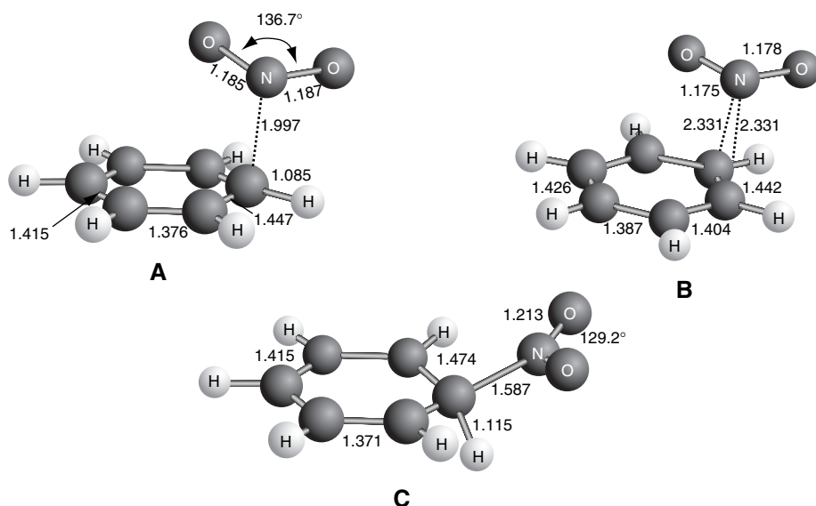
Fig. 9.10. Oriented complexes and nitrocyclohexadienylum intermediate in the nitration of benzene. Adapted from J. Am. Chem. Soc. , 125 , 4836 (2003), by permission of the American Chemical Society.
